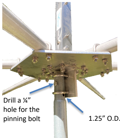
Standard Push up Mast Bracket
