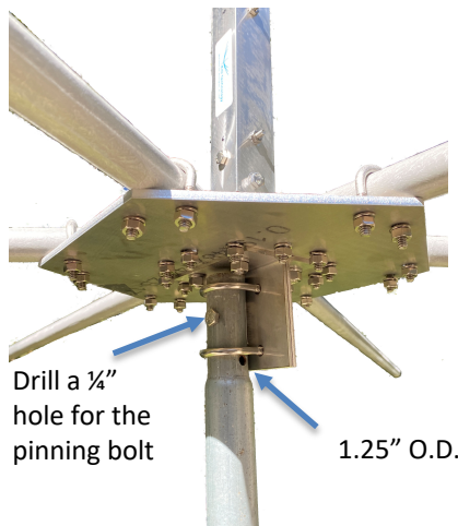
Standard Push up Mast Bracket
